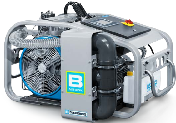
MARINER 320-OX with BeInding Panel, electric motor, 4 filling hoses with nitrox connections (standard)
